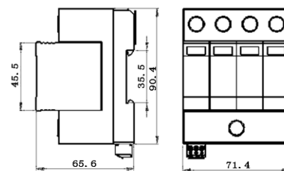
All dimension in mm Dimension drawing
