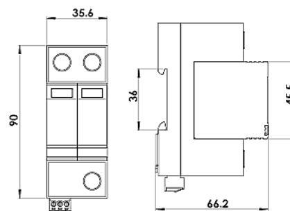
Dimension drawing
