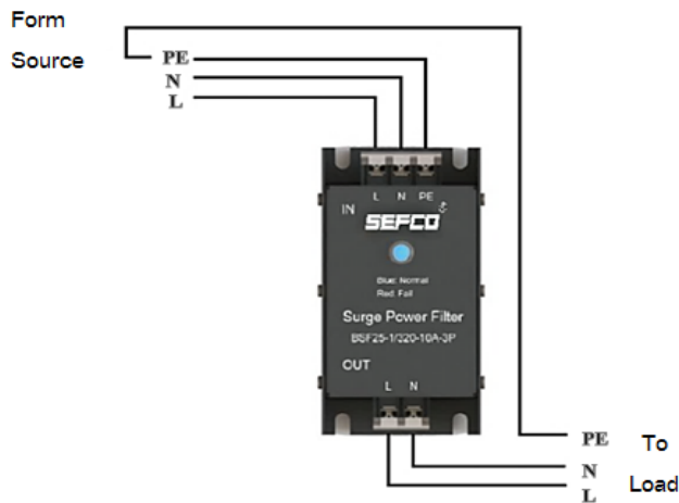
Connection diagram
