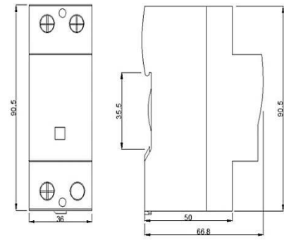
Dimension drawing
